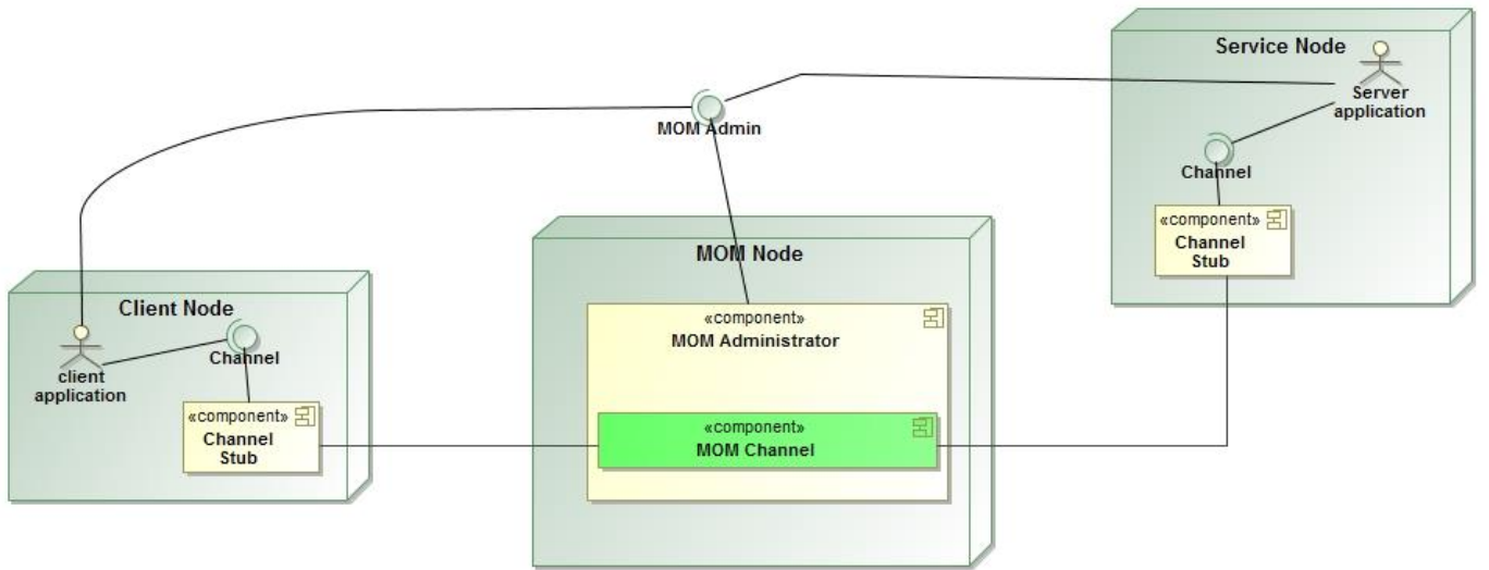
Typical MOM Architecture
